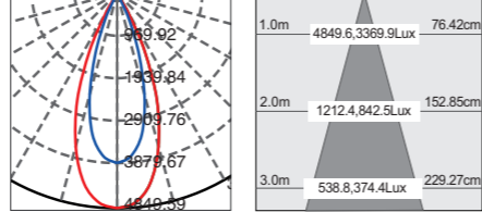
COB 35W 40° Photometric / Luminance
